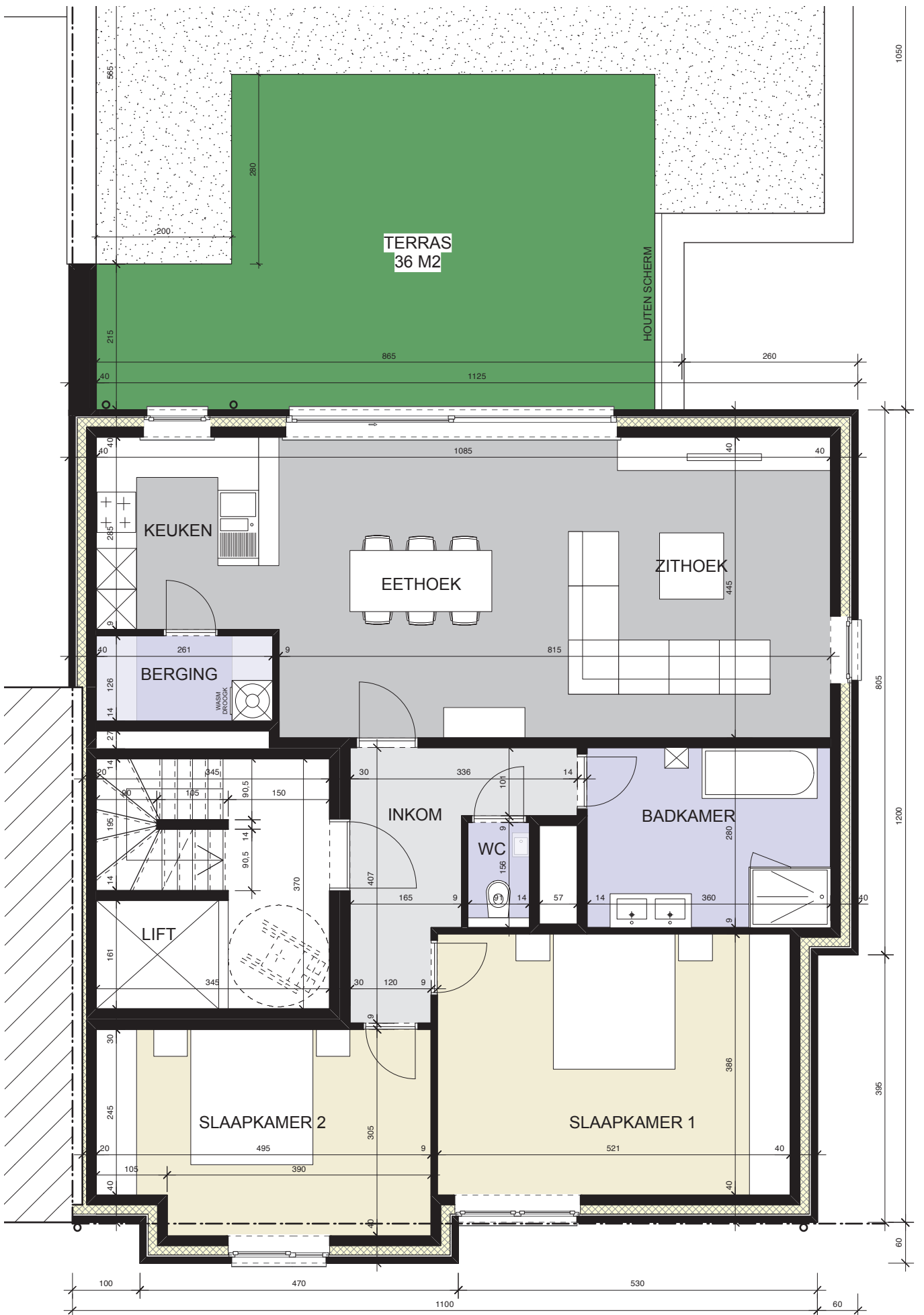
VERDIEPING +1 - SCHAAL 1/75 APPARTEMENT 3 - CA. 113 M2
